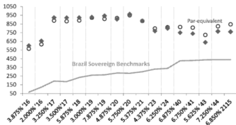
Figure 3: Petrobras' spread curve is inverted beyond 2020
