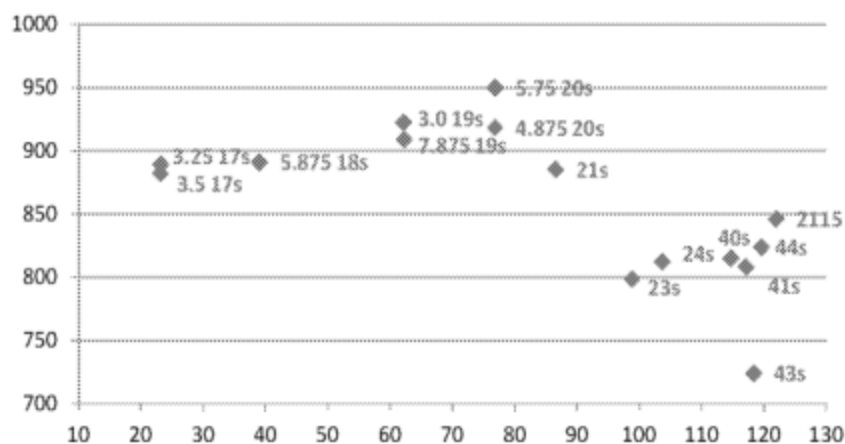
Figure 4: Par-equivalent Spread vs. Cumulative Debt Maturities (USDbn)
