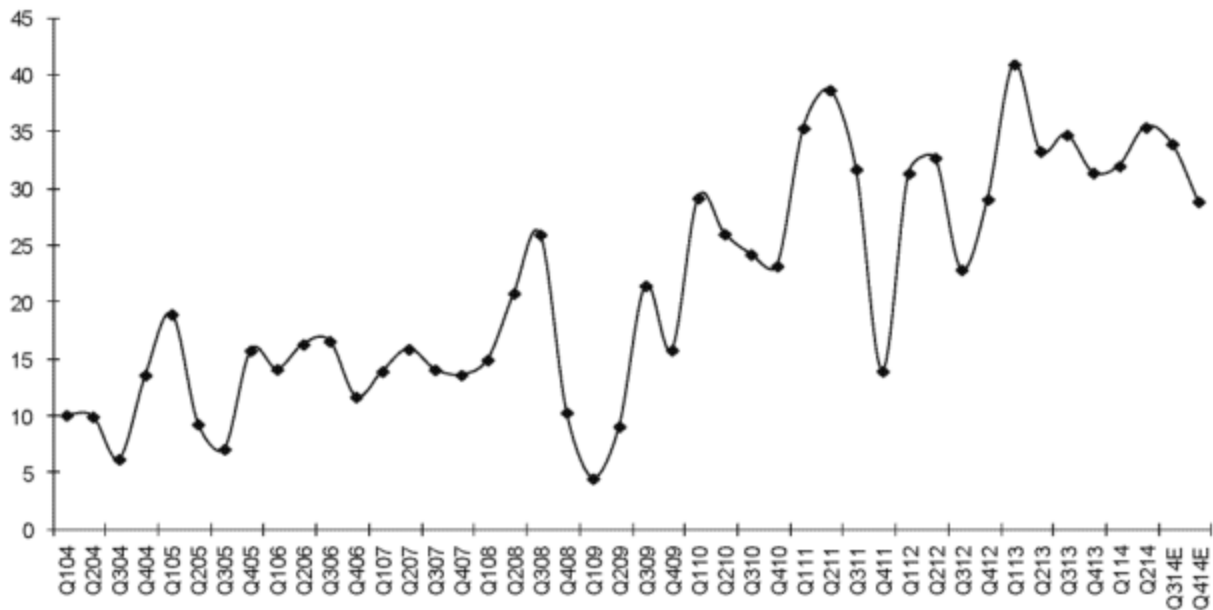
Figure 2: US Propane to Propylene spread (c/lb) in poised to fall in Q3'14 vs Q2'14 due to modestly higher propane prices
