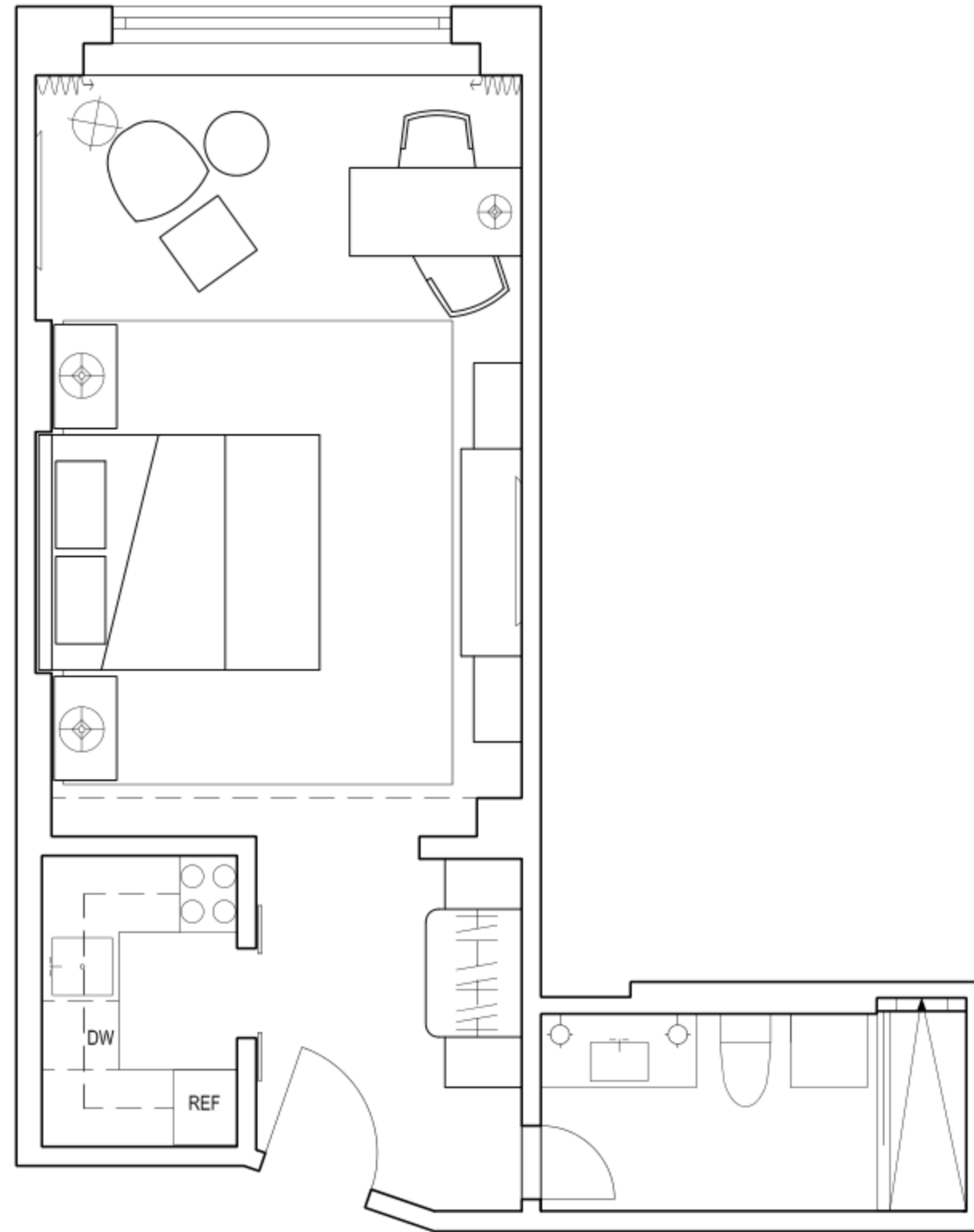
1 RESIDENCE 8A - SHORT TERM 1/4" = 1'-0"
