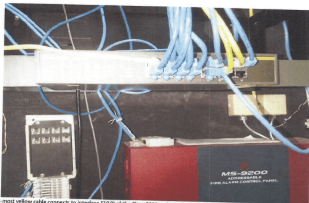
The left-most yellow cable connects to interface FE0/0 of the Cisco 2800 series router. The patch cables in the remaining ports connect to the patch panel below or to wireless devices that distribute internet access to the ranch. The following equipment is not part of the service delivery infrastructure; rather their purpose is to distribute Ethernet to various locations across Zorro Ranch and should be considered part of the distribution infrastructure.
