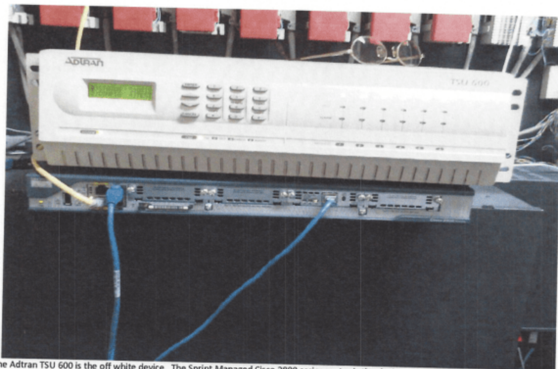
The Adtran TSU 600 is the off white device. The Sprint Managed Cisco 2800 series router is the device with green trim underneath the Adtran TSU 600. The right-most blue cable connects the T1 card on the Cisco Router to the Adtran Tracer in the HVAC room. The yellow cable on the left (Interface FE0/0) connects to the D-Link switch. The D-Link switch is what provides internet access to the network drops throughout the main house.
