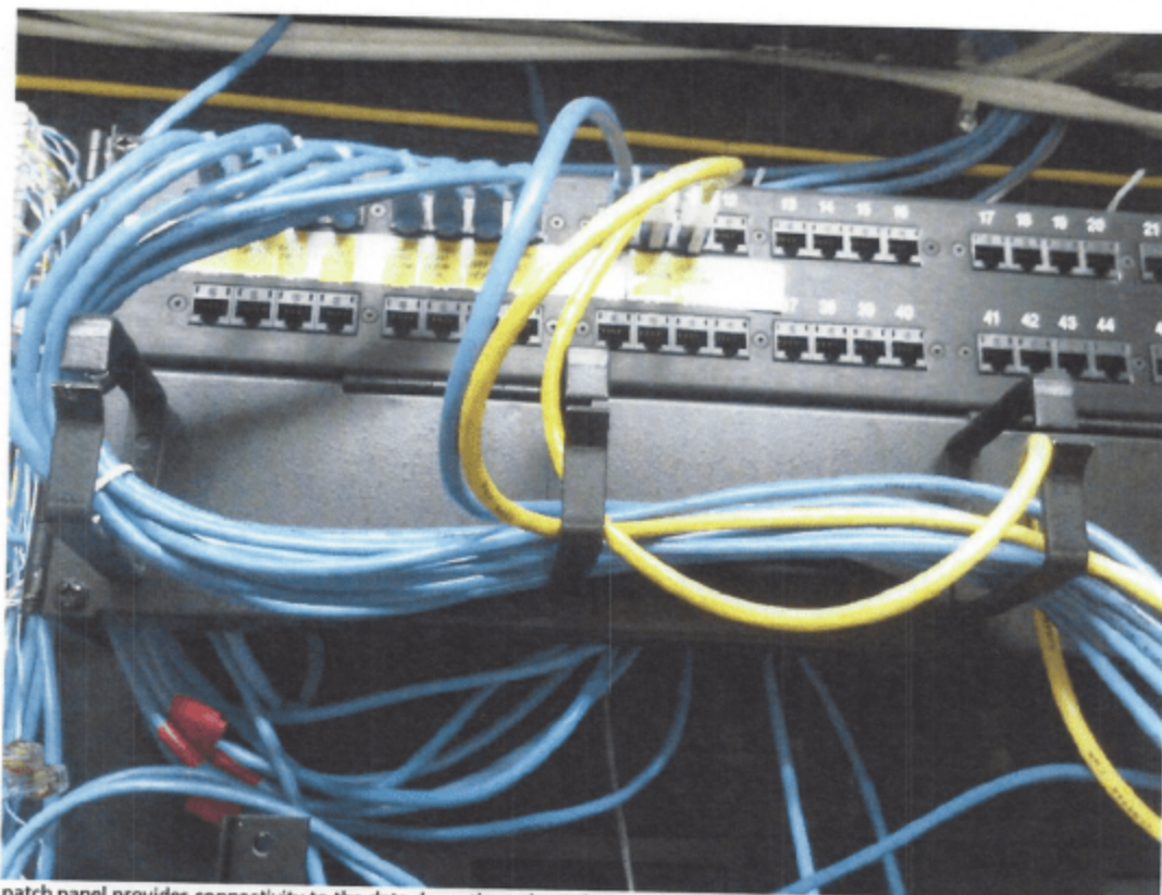
This patch panel provides connectivity to the data drops throughout the main house. The labels indicate where the data drop is physically located. Connecting these ports to the D-Link switch will "light" a drop with internet access.
