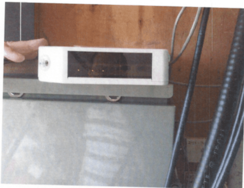
Sprint data T1 card in the generator room of transmitter shack 75 at Sandia Crest. Notice that all lights on the front are green. In the event of an outage, you will want to note if there are any amber or red LEDs illuminated on either of these cards.
