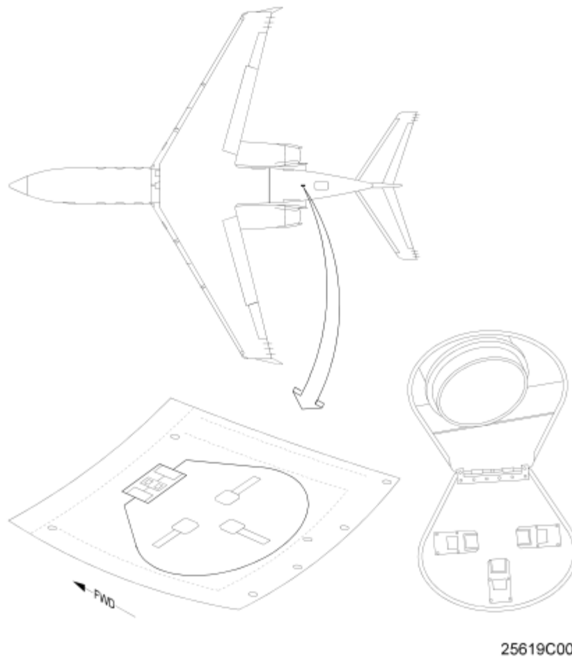
External Starting Air Connection Figure 9
