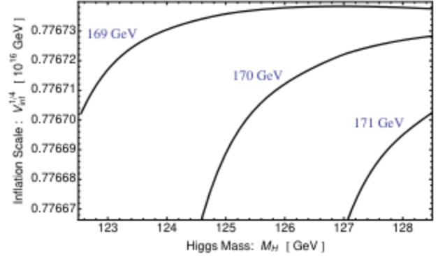
FIG. 1: The predicted energy scale of inflation, V_{\text{inf}}^{1/4} , over a range of Higgs boson masses ( M_H ), for three values of the top quark mass ( M_t ), and in the Landau gauge, \xi_{\text{gf}} = 0 .
