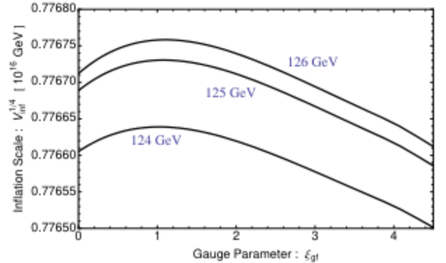
FIG. 2: The energy scale of inflation, V_{\text{inf}} , as the gauge parameter, \xi_{\text{gf}} , varies. We fix M_t = 170 GeV and show three values of M_H .
